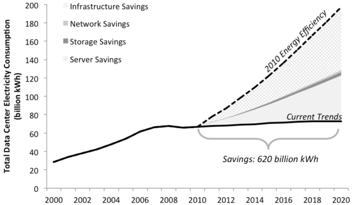
Figure 1.1: Power consumption of data centers
