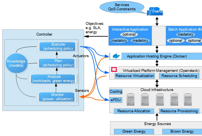
Figure 7.1: Perspective model
