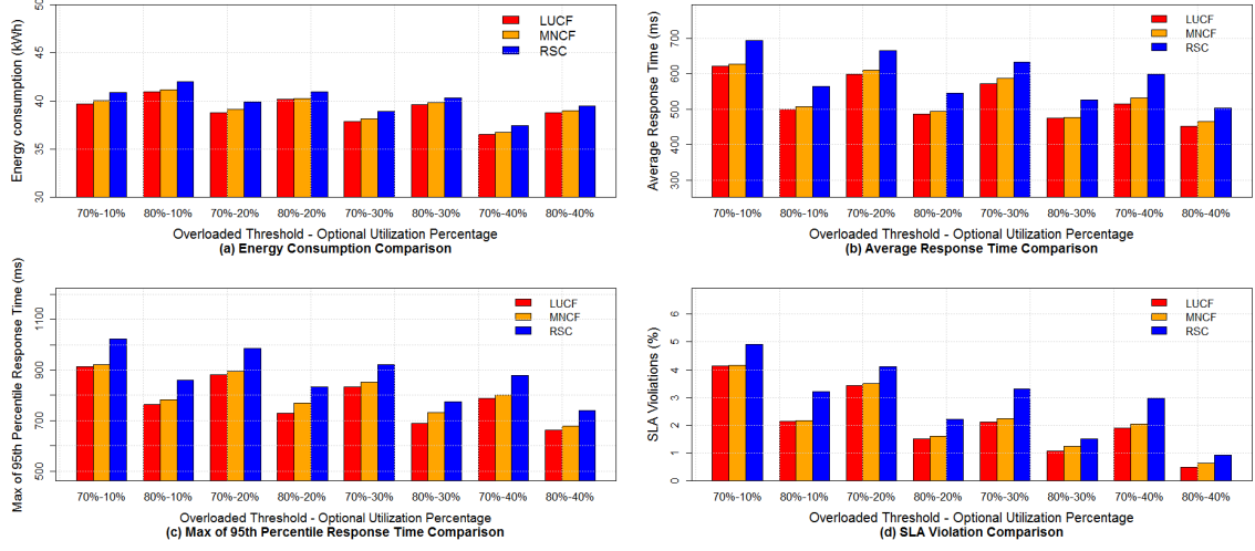
Figure 5.6: Performance Comparison of Proposed Policies
